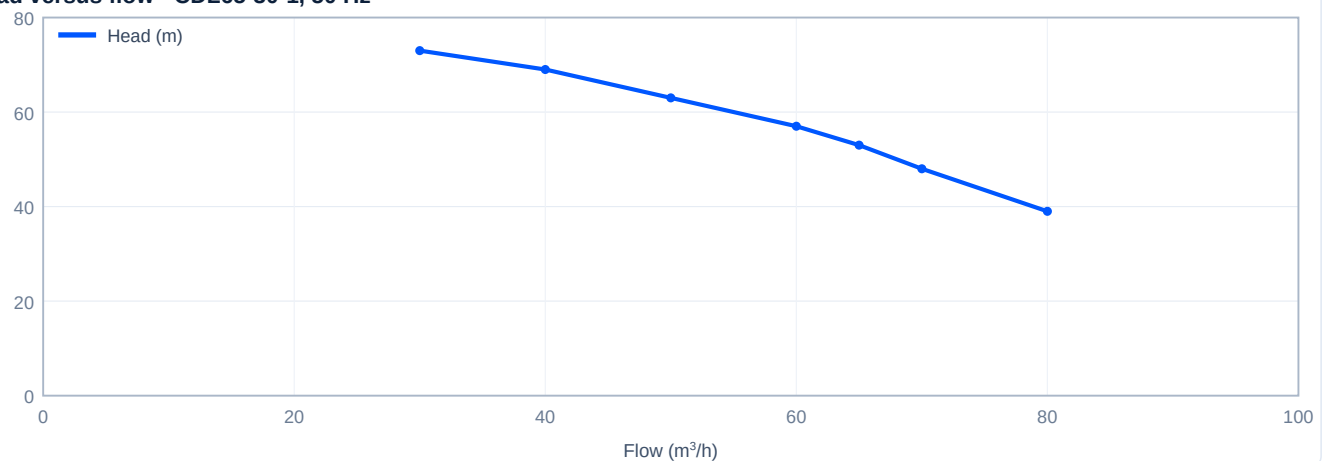
Head versus flow - CDL65-30-1, 50 Hz
