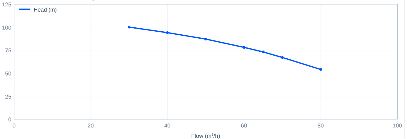
Head versus flow - CDL65-40-1, 50 Hz
