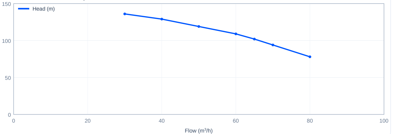
Head versus flow - CDL65-50, 50 Hz
