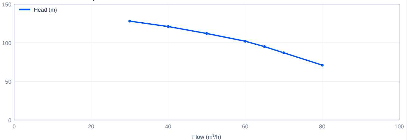
Head versus flow - CDL65-50-1, 50 Hz
