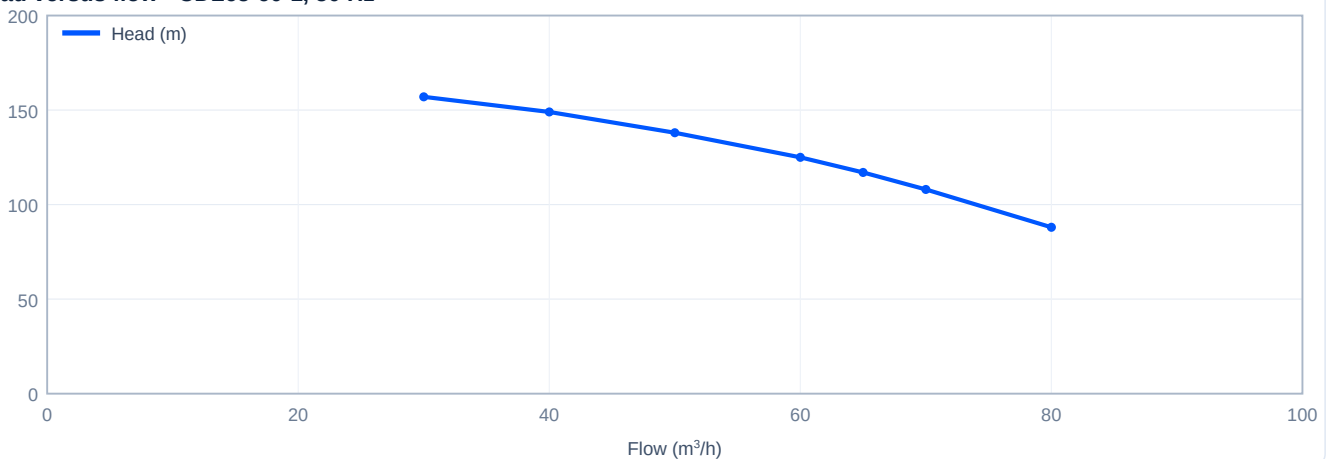
Head versus flow - CDL65-60-1, 50 Hz
