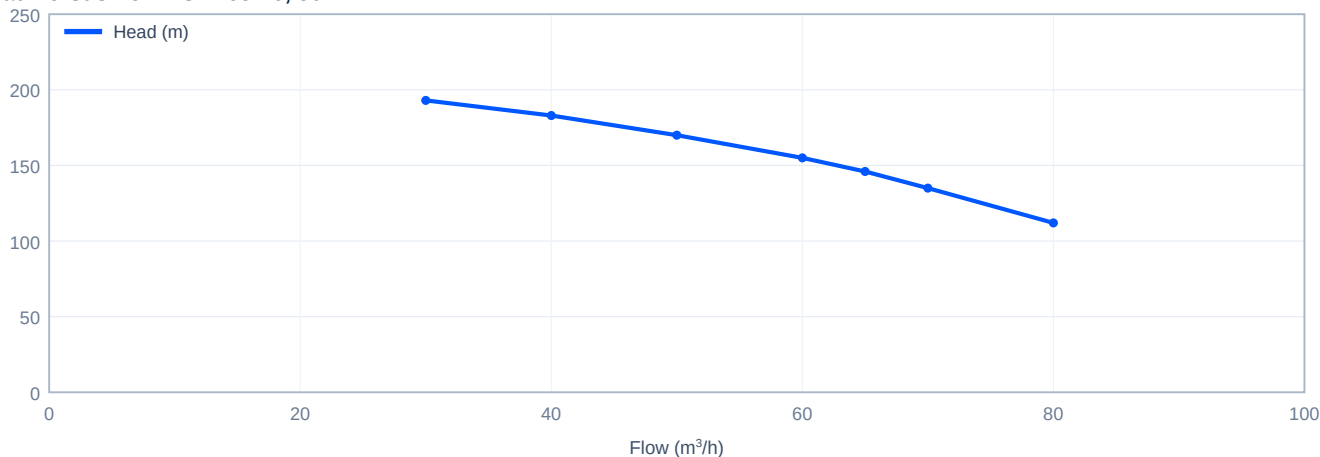
Head versus flow - CDL65-70, 50 Hz
