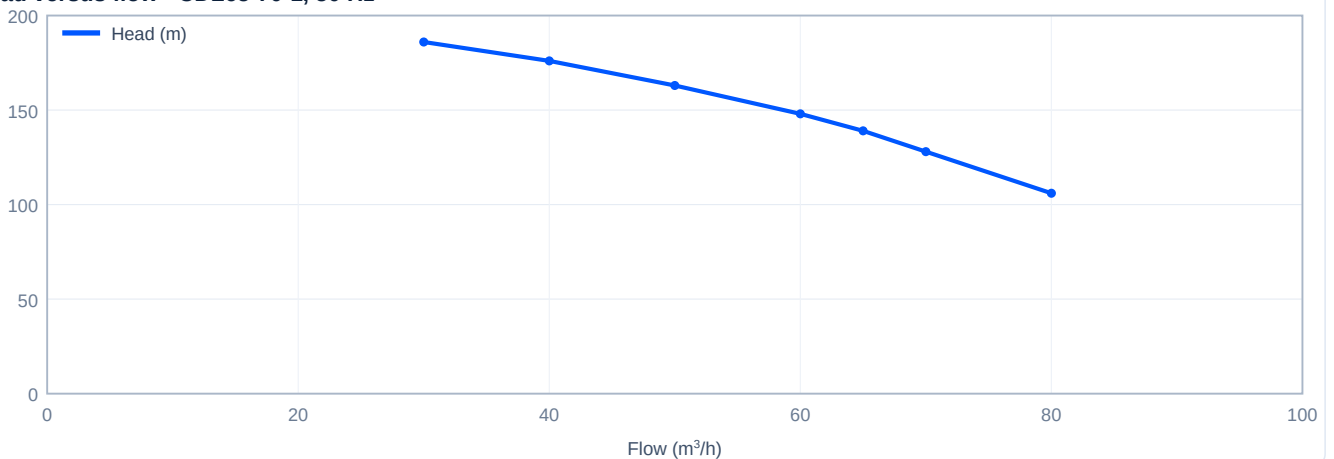
Head versus flow - CDL65-70-1, 50 Hz
