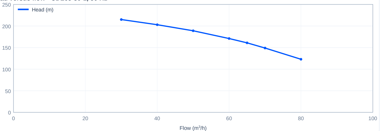
Head versus flow - CDL65-80-1, 50 Hz
