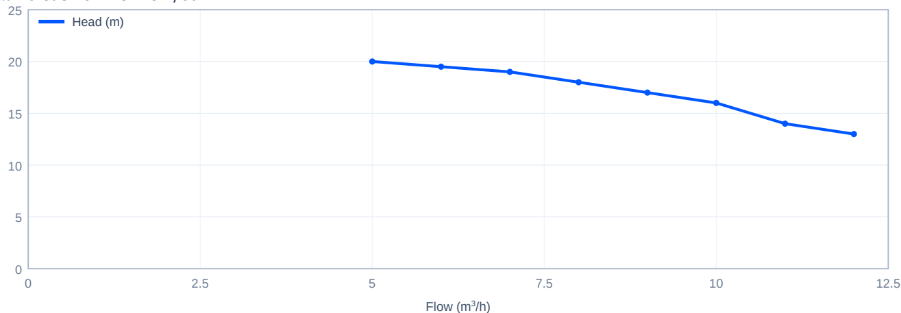
Head versus flow - CDL8-2, 50 Hz
