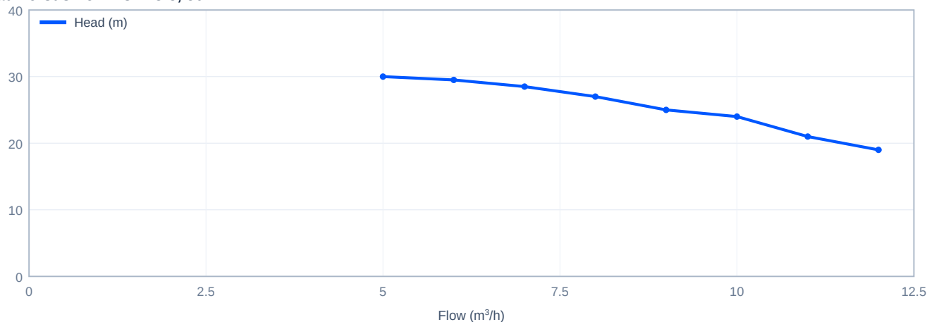
Head versus flow - CDL8-3, 50 Hz
