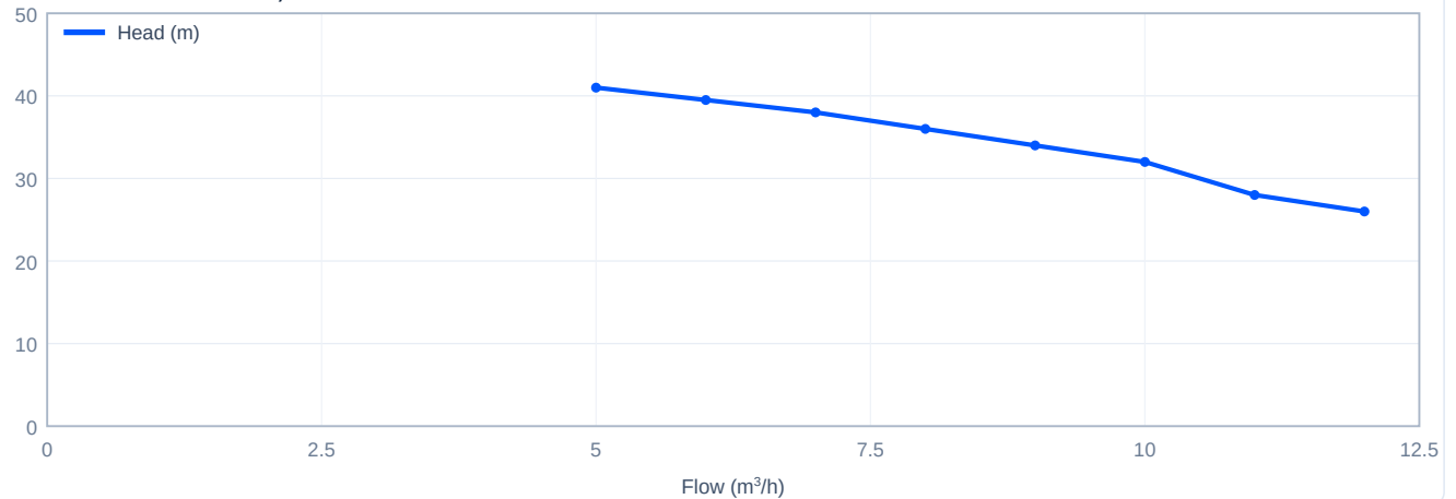
Head versus flow - CDL8-4, 50 Hz
