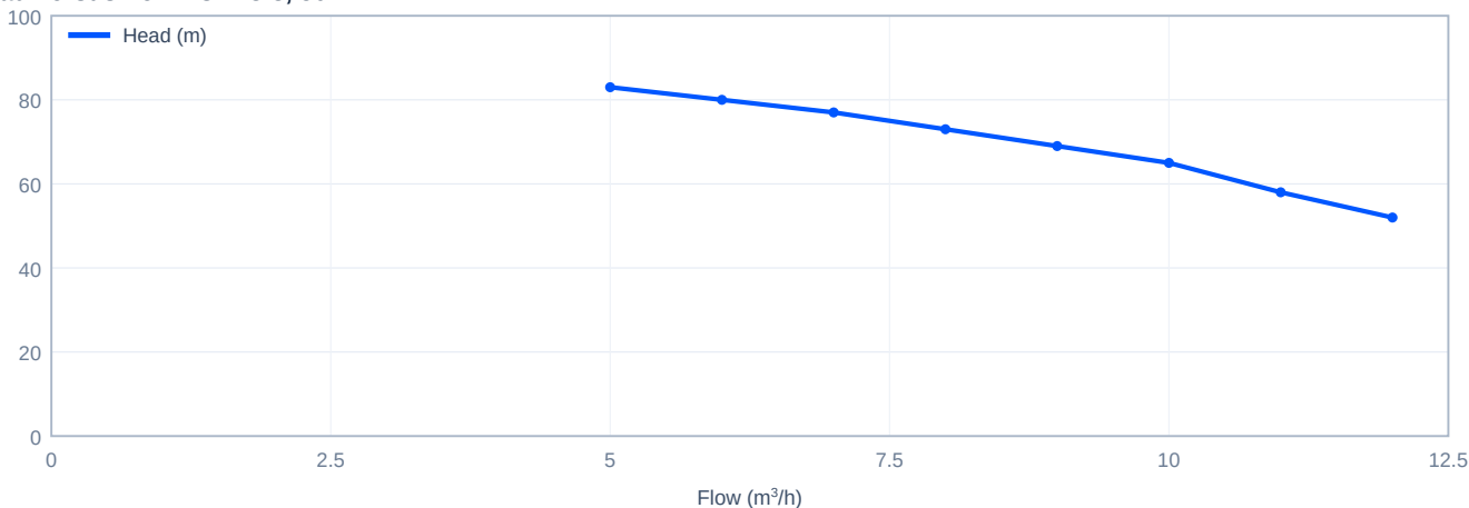
Head versus flow - CDL8-8, 50 Hz
