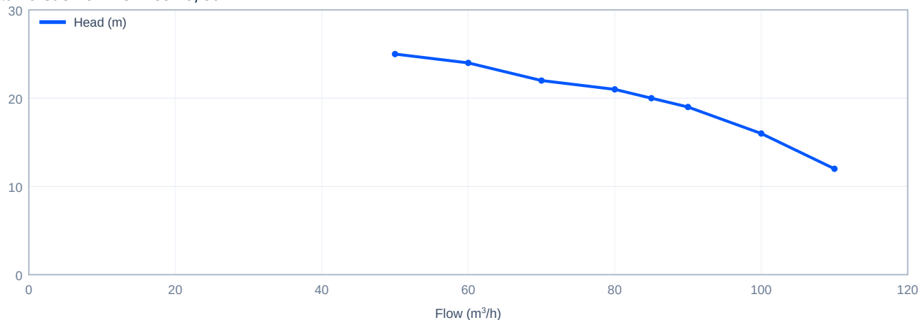
Head versus flow - CDL85-10, 50 Hz
