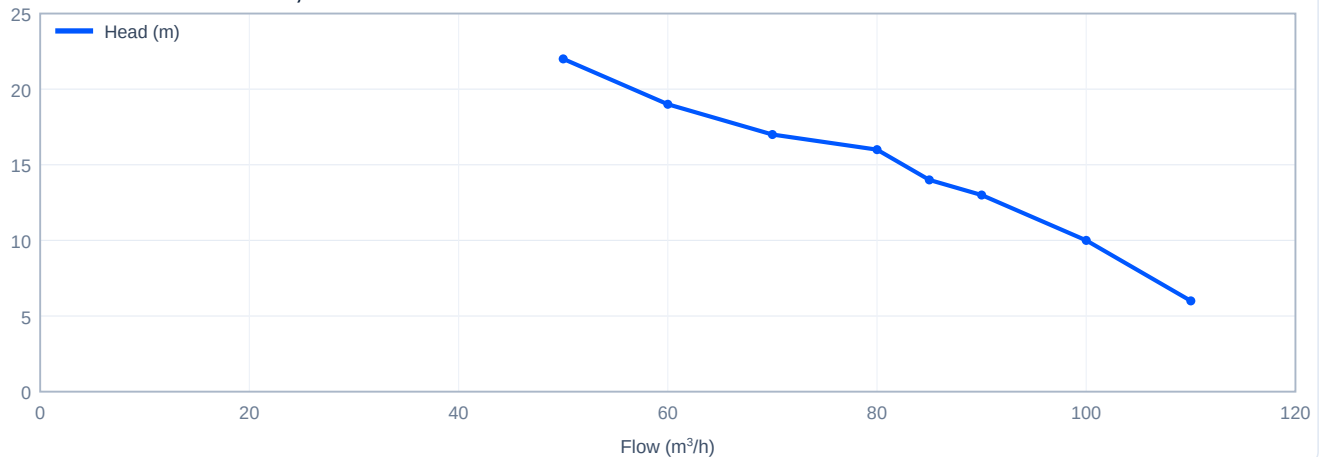
Head versus flow - CDL85-10-1, 50 Hz
