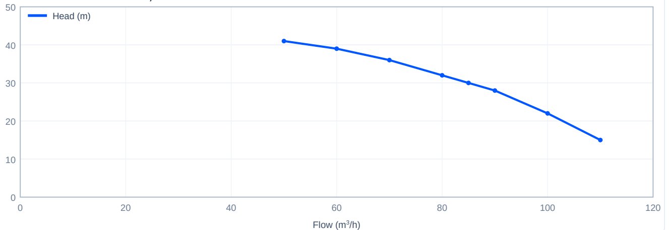
Head versus flow - CDL85-20-2, 50 Hz
