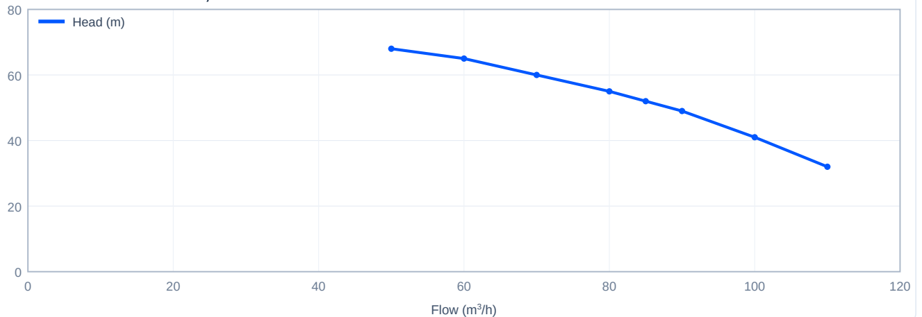
Head versus flow - CDL85-30-2, 50 Hz
