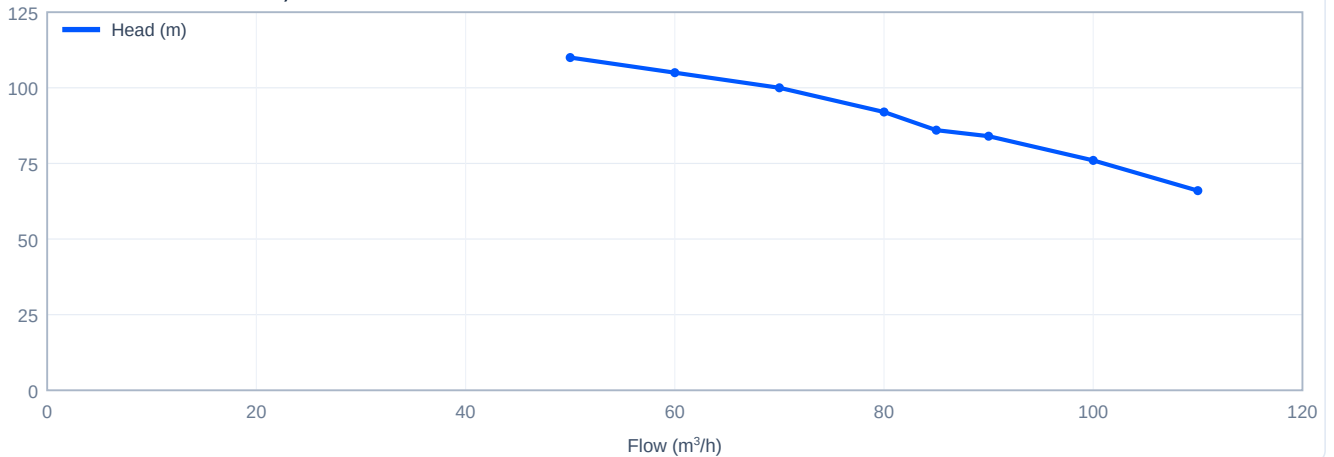
Head versus flow - CDL85-40, 50 Hz
