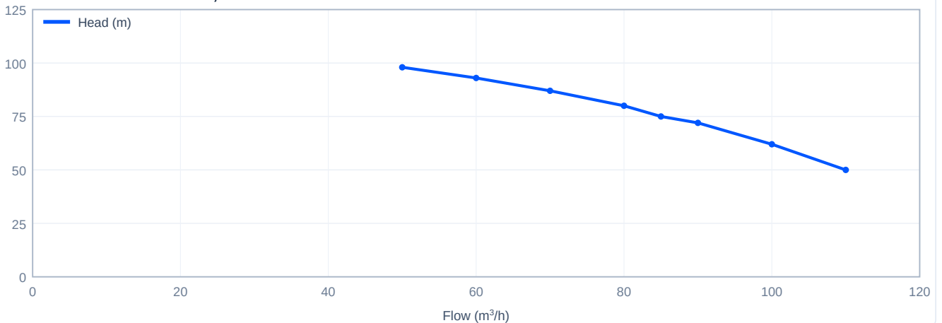
Head versus flow - CDL85-40-2, 50 Hz
