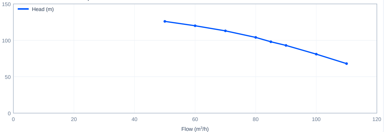
Head versus flow - CDL85-50-2, 50 Hz
