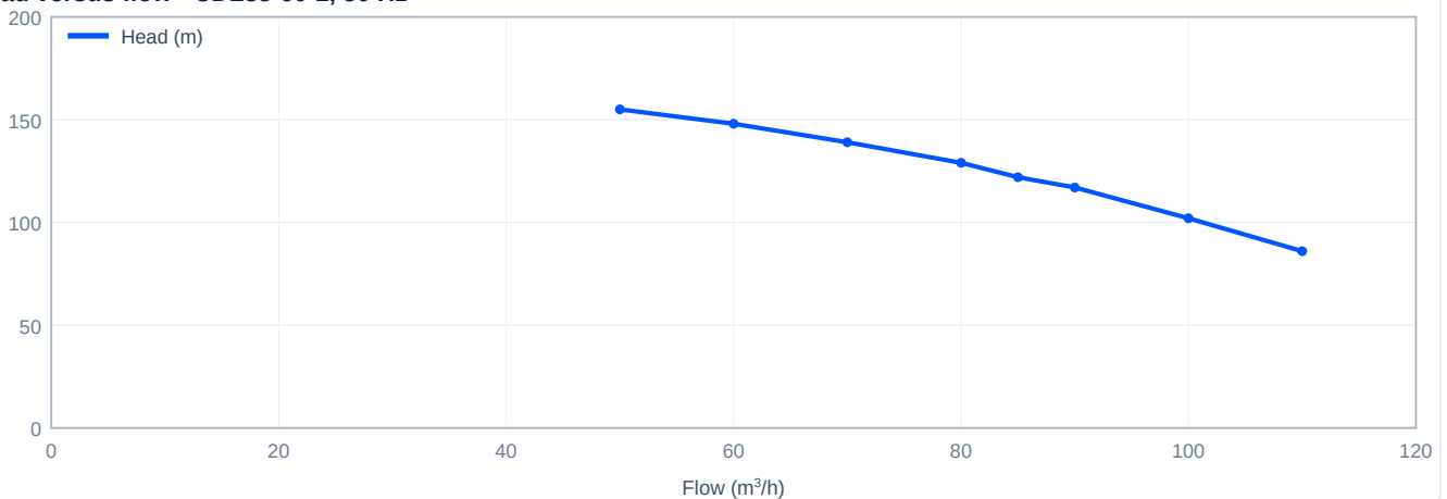
Head versus flow - CDL85-60-2, 50 Hz
