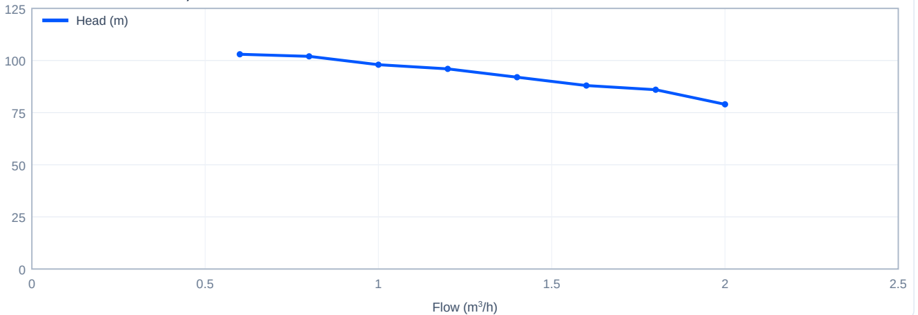
Head versus flow - CDL1-12, 60 Hz
