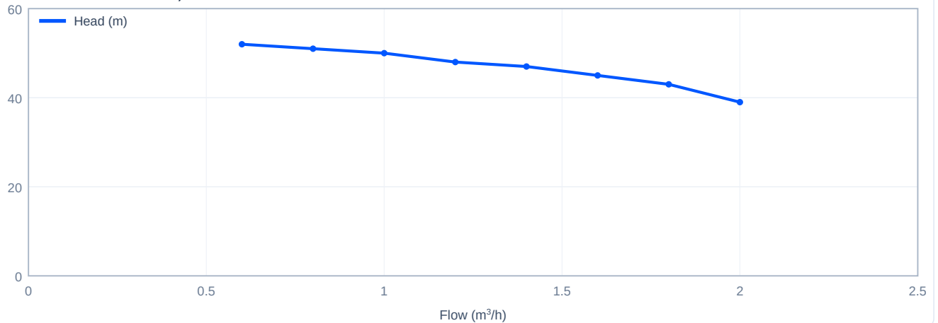
Head versus flow - CDL1-6, 60 Hz
