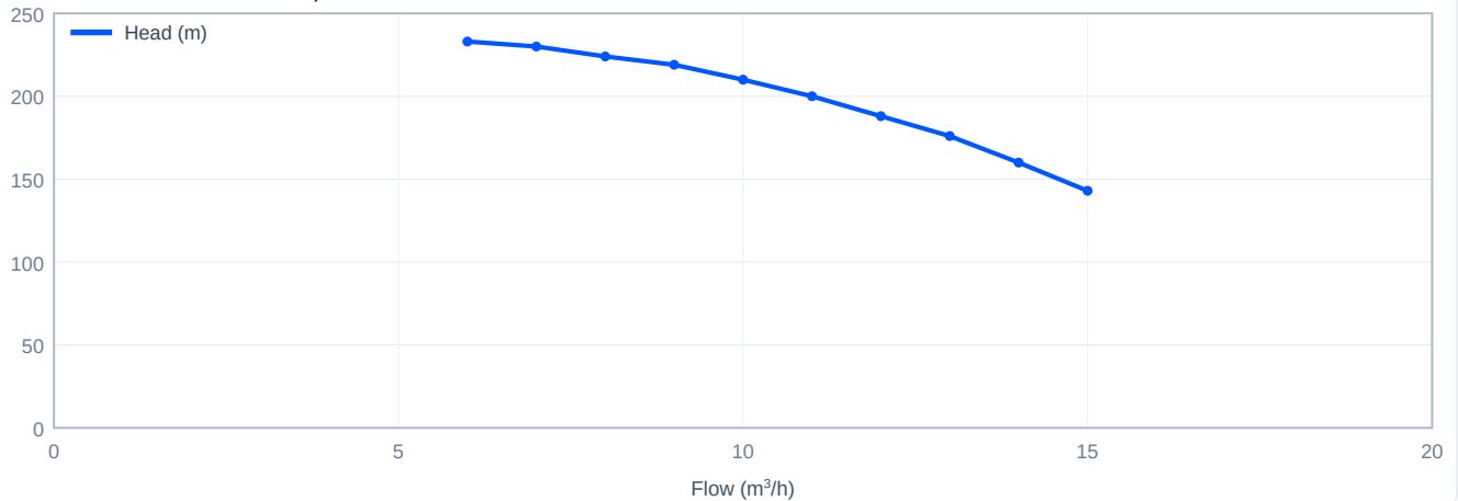
Head versus flow - CDL10-16, 60 Hz
