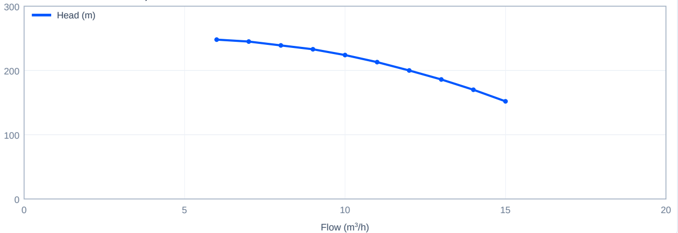
Head versus flow - CDL10-17, 60 Hz
