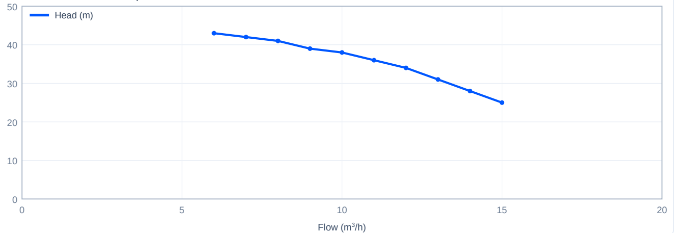
Head versus flow - CDL10-3, 60 Hz
