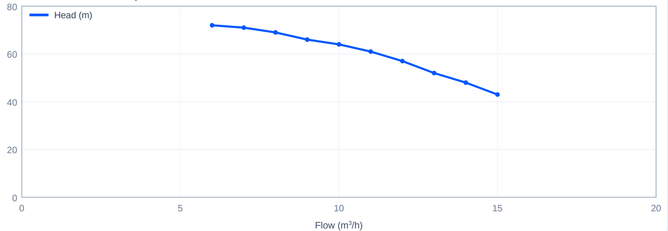
Head versus flow - CDL10-5, 60 Hz
