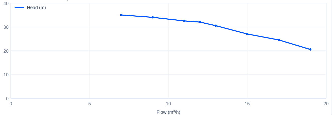
Head versus flow - CDL12-2, 60 Hz
