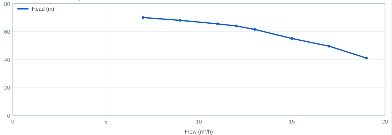
Head versus flow - CDL12-4, 60 Hz
