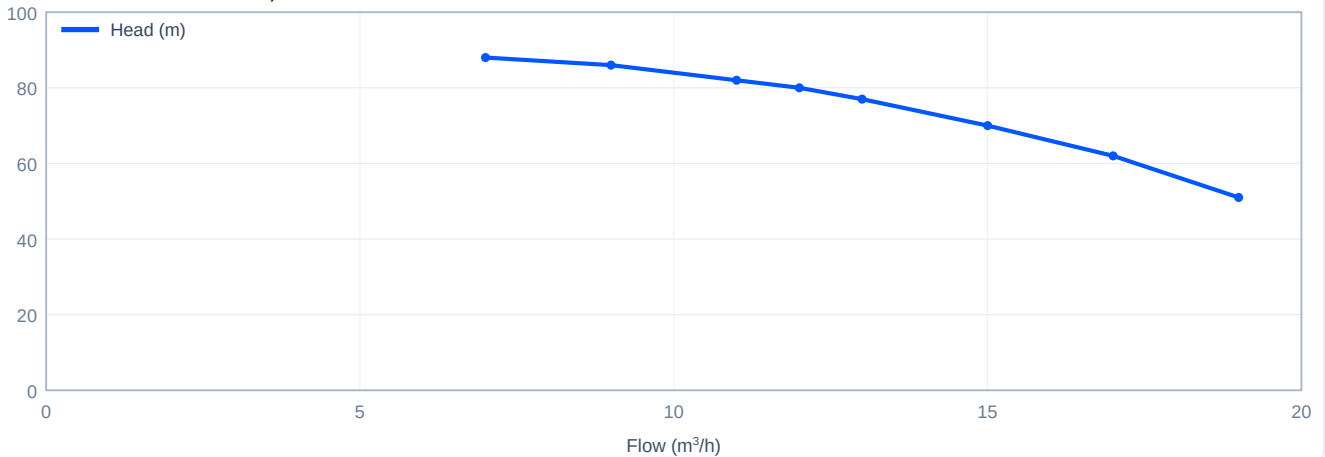
Head versus flow - CDL12-5, 60 Hz
