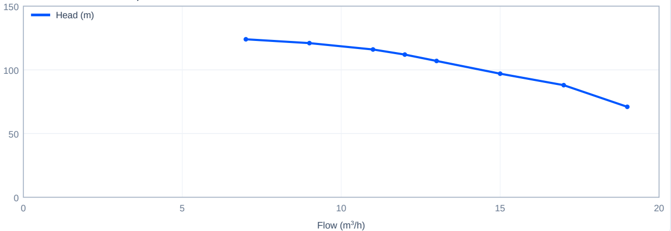
Head versus flow - CDL12-7, 60 Hz
