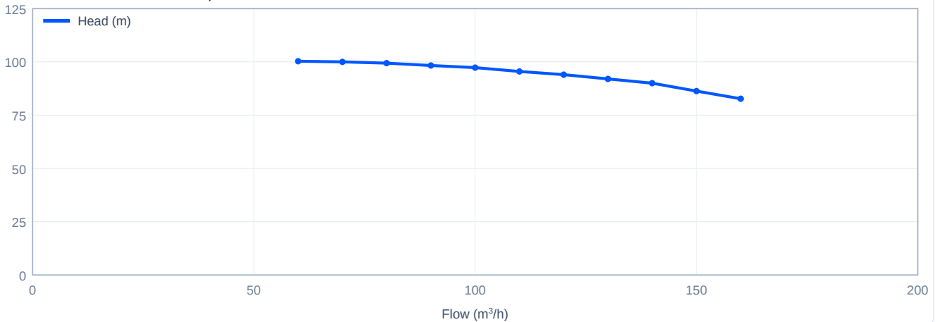
Head versus flow - CDL120-30, 60 Hz
