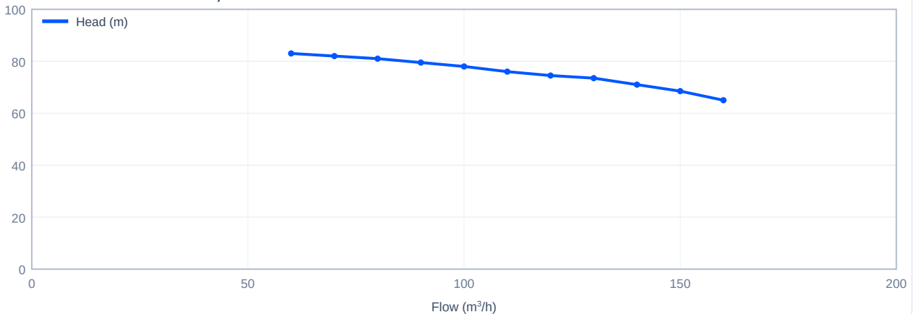
Head versus flow - CDL120-30-2, 60 Hz
