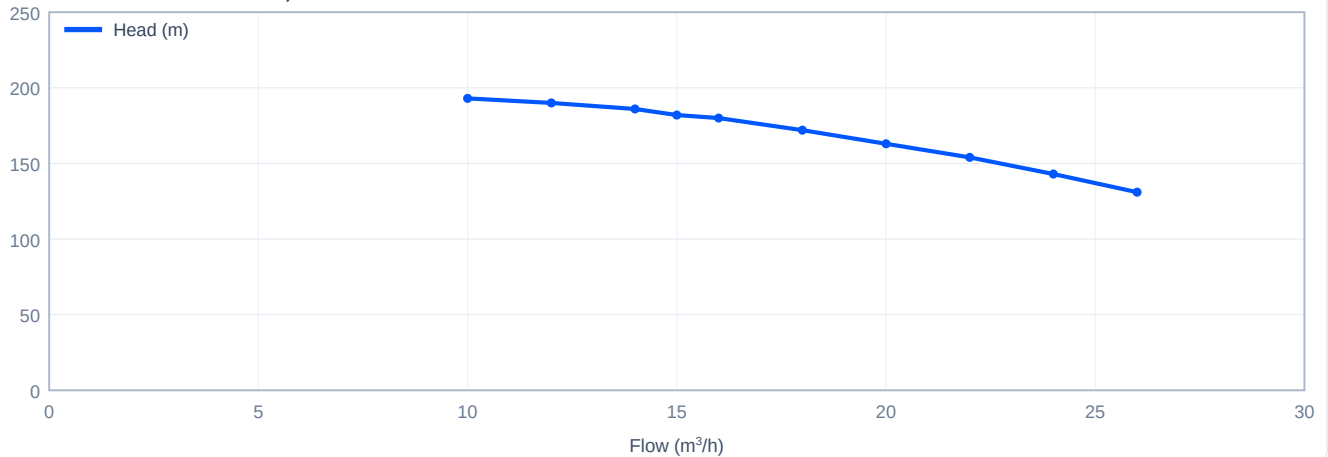
Head versus flow - CDL15-10, 60 Hz
