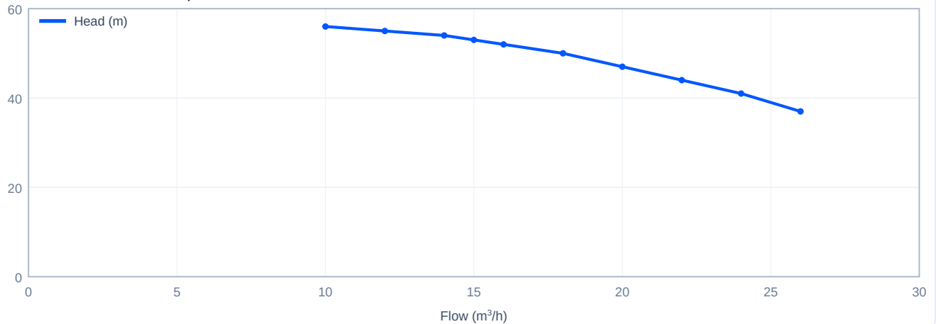
Head versus flow - CDL15-3, 60 Hz
