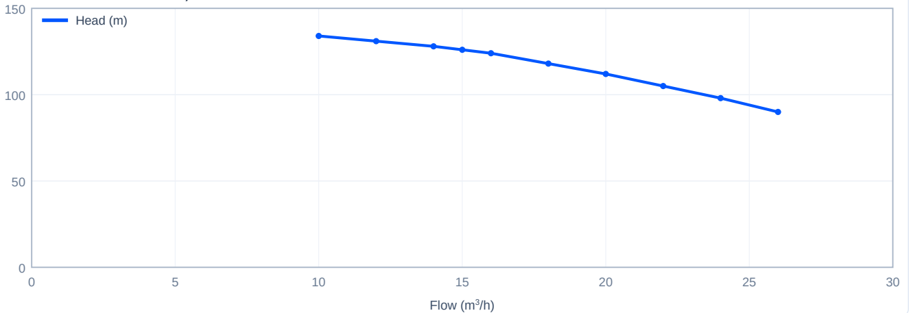
Head versus flow - CDL15-7, 60 Hz
