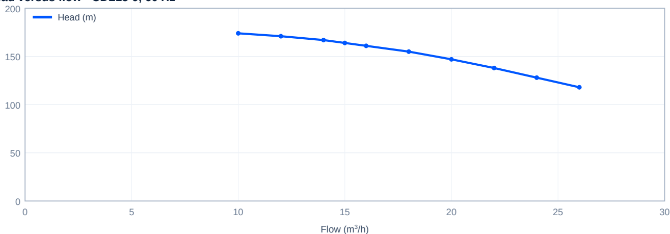
Head versus flow - CDL15-9, 60 Hz
