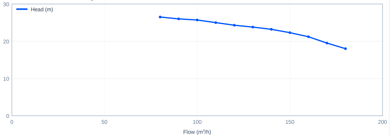
Head versus flow - CDL150-10-1, 60 Hz
