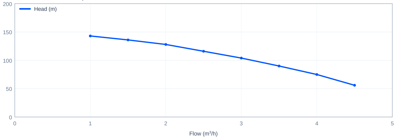
Head versus flow - CDL2-11, 60 Hz
