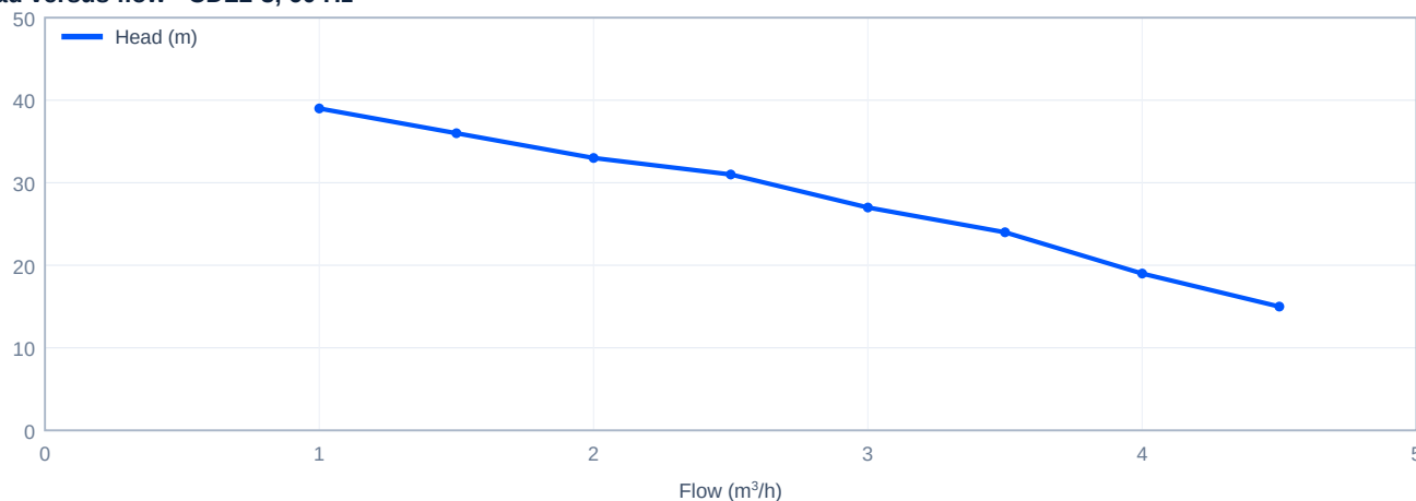
Head versus flow - CDL2-3, 60 Hz
