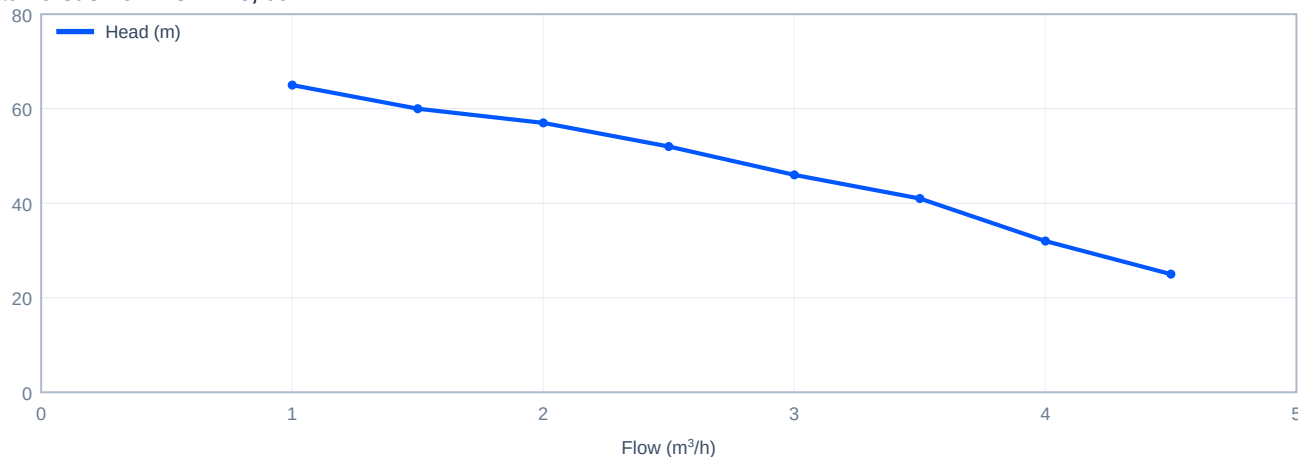
Head versus flow - CDL2-5, 60 Hz
