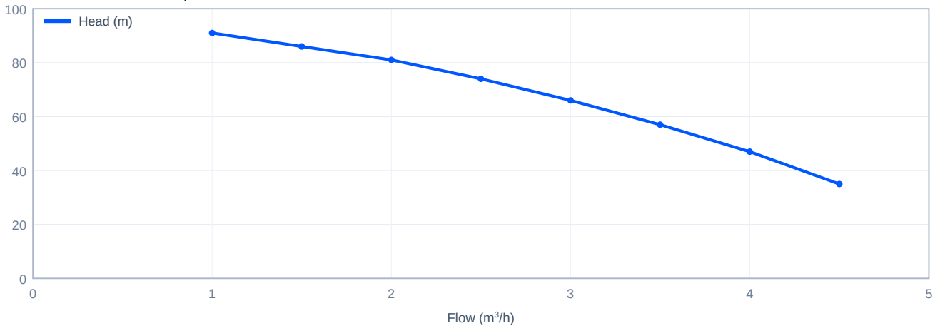
Head versus flow - CDL2-7, 60 Hz
