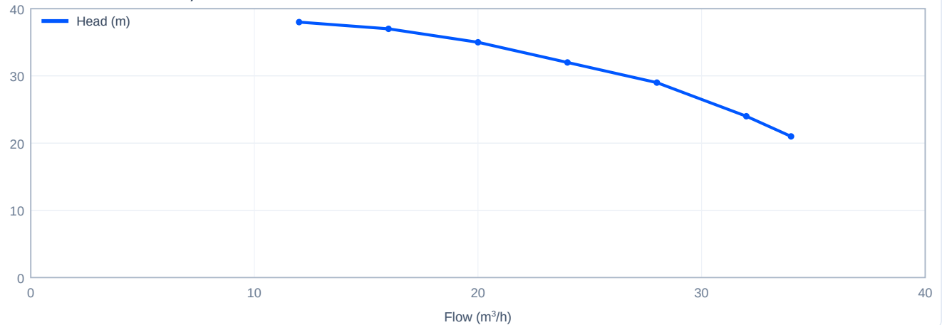
Head versus flow - CDL20-2, 60 Hz
