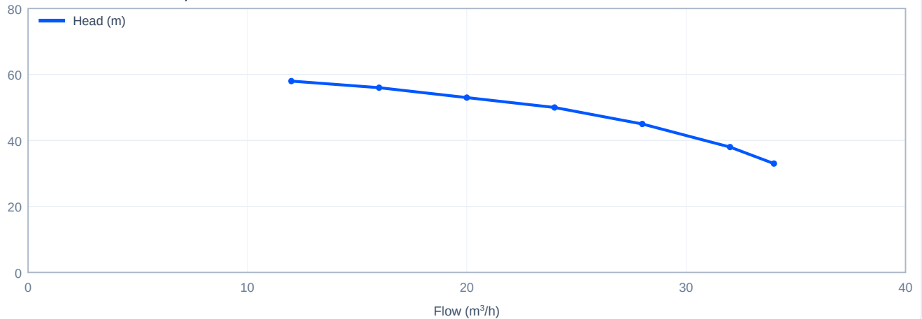
Head versus flow - CDL20-3, 60 Hz
