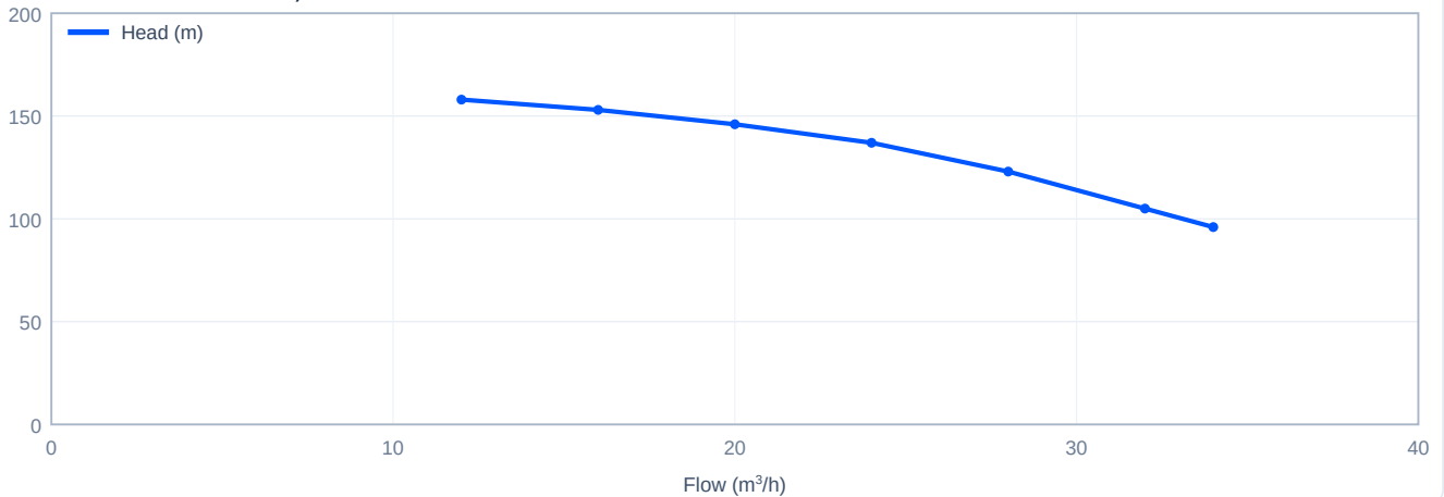
Head versus flow - CDL20-8, 60 Hz
