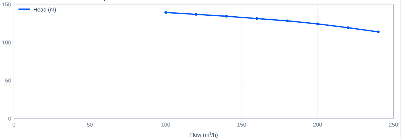
Head versus flow - CDL200-30-A-B, 60 Hz
