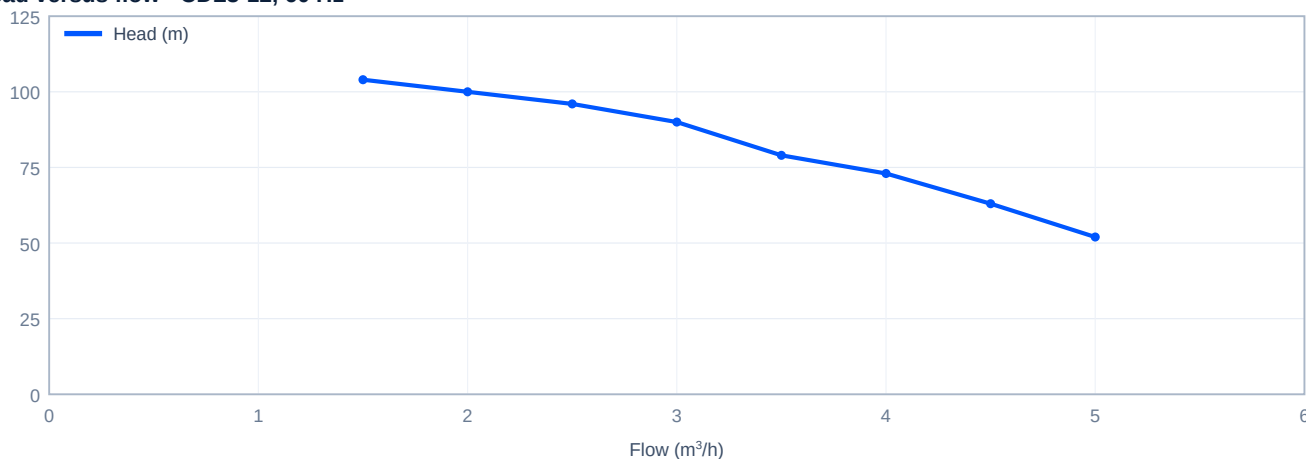
Head versus flow - CDL3-12, 60 Hz
