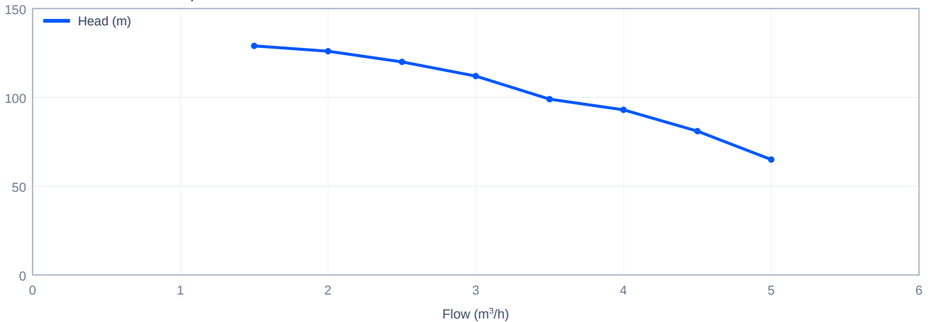
Head versus flow - CDL3-15, 60 Hz
