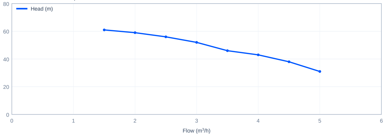
Head versus flow - CDL3-7, 60 Hz
