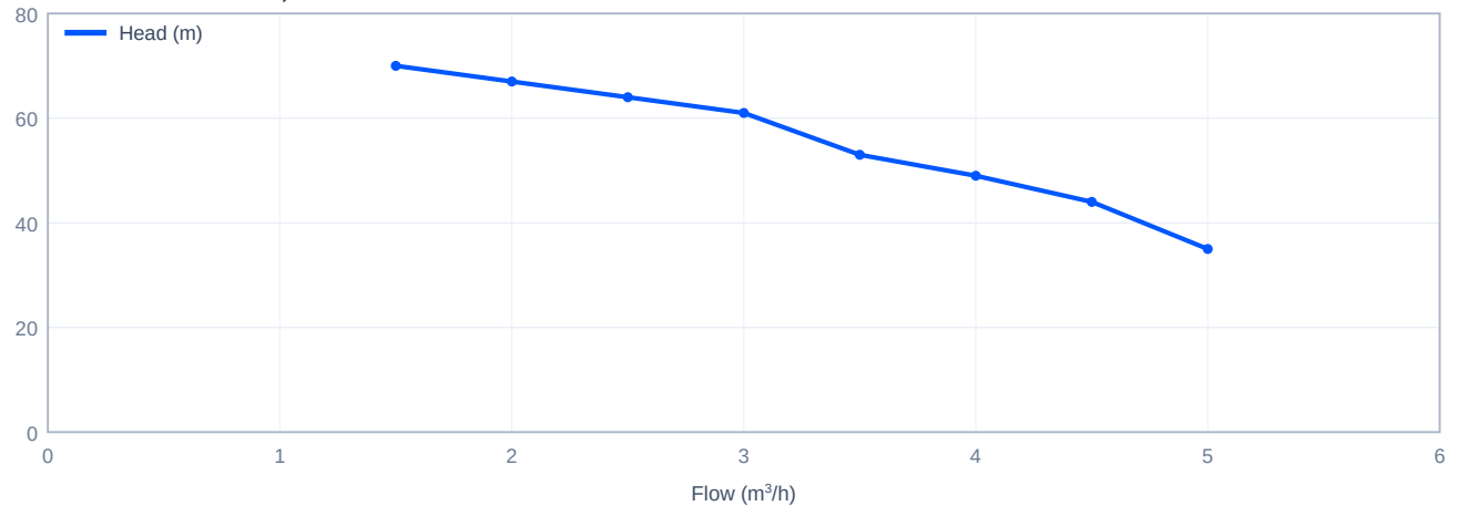
Head versus flow - CDL3-8, 60 Hz
