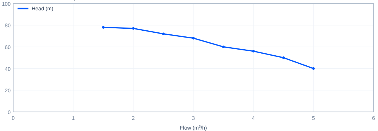
Head versus flow - CDL3-9, 60 Hz
